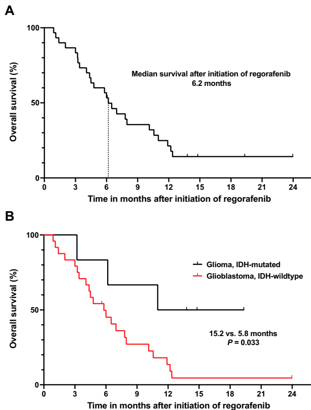
Fig. 3 Kaplan–Meier plots for the median overall survival of all patients (A), and patients stratified according to the IDH-mutation status (B). Patients with an IDH-mutant glioma had a significantly 2.6-fold longer overall survival than patients with an IDH-wildtype (i.e., glioblastoma) (15.2 vs. 5.8 months; P=0.033 )
