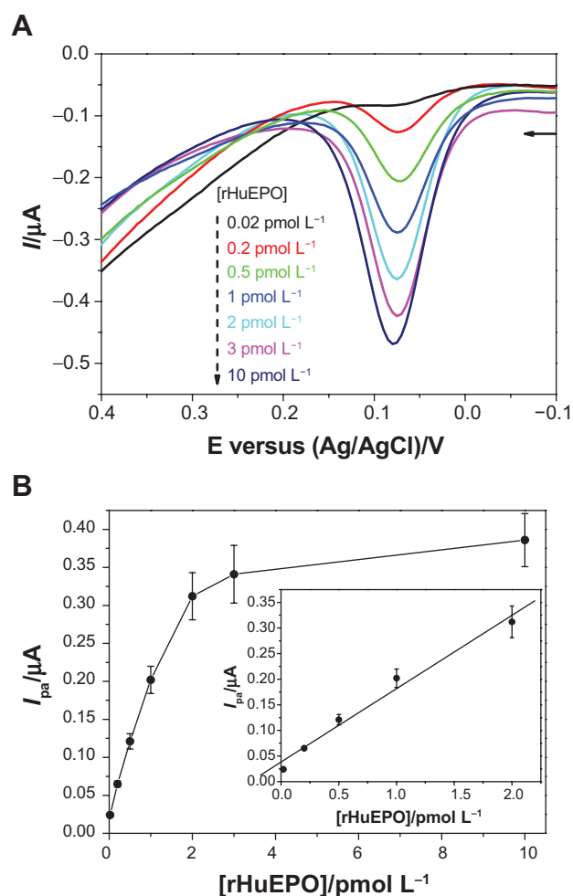
Figure 4 (A) Differential pulse voltammograms for the detection of different concentrations of rHuEPO. (B) Plots of the I_{pa} against the rHuEPO concentration ( 0.02\text{--}10 \text{ pmol L}^{-1} ). The inset shows the linear plots at concentrations of 0.02, 0.2, 0.5, 1.0, and 2.0 \text{pmol L}^{-1} .
