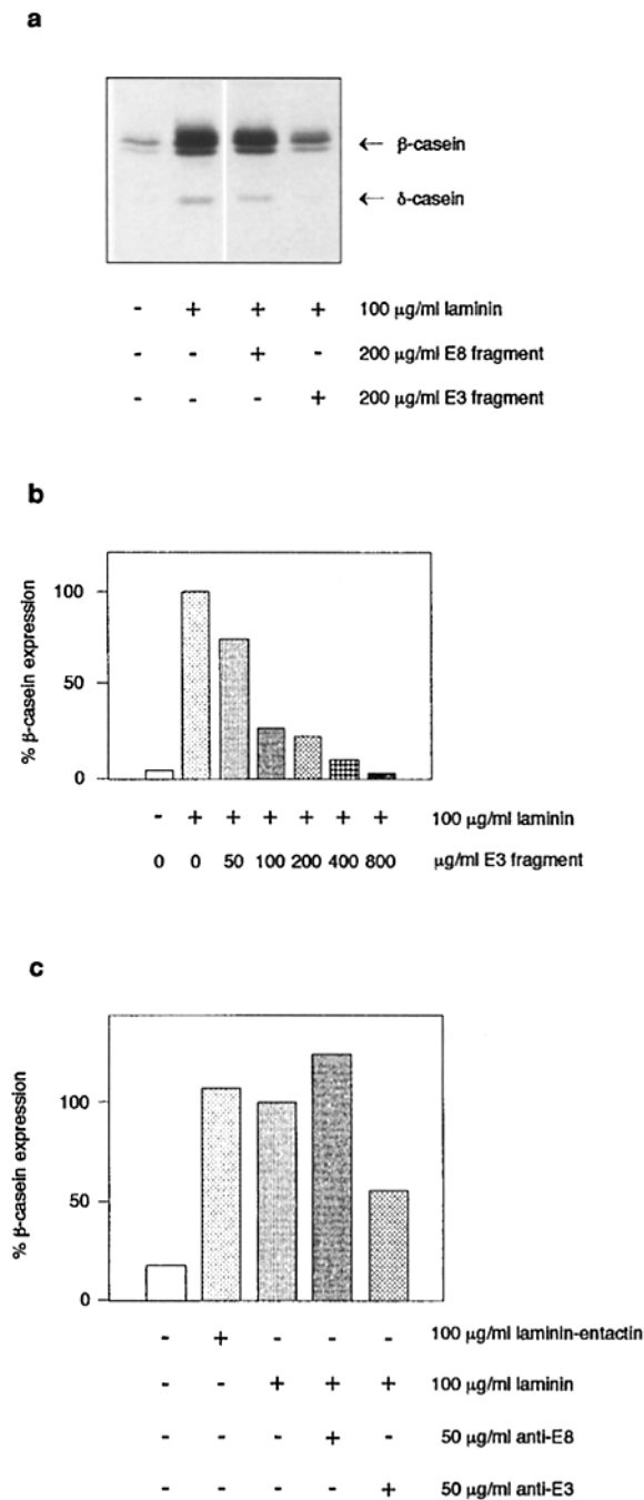
Figure 6. The laminin signaling domain is contained within the E3 region. (a) Mammary cells cultured in hormone-containing medium for 3.5 d synthesized \beta -casein in the presence of 100 \mu\text{g/ml} laminin. This was competitively blocked by 200 \mu\text{g/ml} E3 fragment, but not by 200 \mu\text{g/ml} E8 fragment. (b) Dose response of the inhibition by E3 fragment of laminin-induced casein expression. The results in this experiment and in c were obtained by quantitative analysis of immune precipitates prepared as in Fig. 3, using a Fuji BAS 2000 Bio Imaging Analyzer. The amounts of \beta -casein present in each experimental condition are expressed as a percentage of the total \beta -casein induced by 100 \mu\text{g/ml} laminin alone. (c) The induction of \beta -casein expression by laminin was blocked by antibodies raised against the E3 domain, but not against the E8 domain. These antibodies were raised against pure laminin domains, and IgG fractions were finally purified by affinity chromatography on a laminin column.
