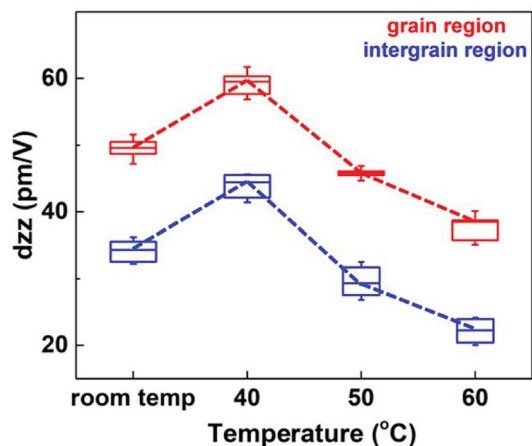
Fig. 6 The evolution of the local piezoelectric coefficients d_{zz} with different temperatures for both the grain and intergrain regions. It illustrates that the maximum d_{zz} is obtained at 40 °C, and the identical changing tendency with the temperature for two different regions can also be observed.
