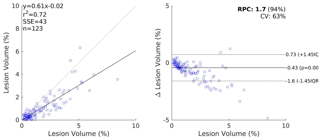
Fig. 15. Scatter and Bland-Altman plots comparing of the lesion volumes (as a percentage of intracranial volume) from LGA to those from the reference segmentations.
