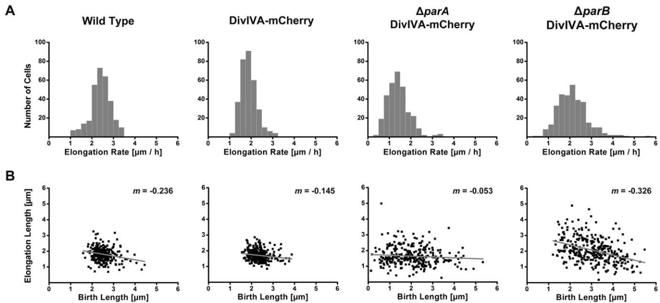
Figure 1. Chromosome segregation defects lead to altered growth in C. glutamicum . (A) Distribution of elongation rates of wild type, DivIVA-mCherry, \Delta\text{parA} DivIVA-mCherry and \Delta\text{parB} DivIVA-mCherry mutant cells. ( n \geq 300 ). (B) Association of birth lengths and elongation lengths in DivIVA-mCherry, \Delta\text{parA} DivIVA-mCherry and \Delta\text{parB} DivIVA-mCherry. In wild type and DivIVA-mCherry cells the birth length and elongation length are associated. In the absence of parA or parB , more variation in the length of the cell at birth and the cell length before division is observed. Negative correlation between birth and elongation lengths indicates a size-based cell cycle regulatory mechanism (grey line). Regression line slope is shown on top right. ( n \geq 300 ).
