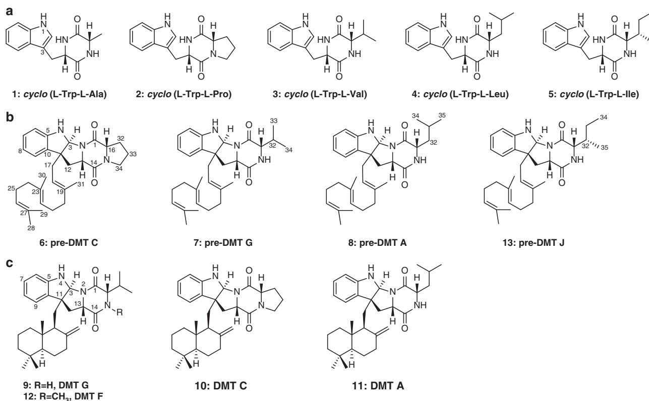
Fig. 1 Chemical structures of compounds 1–13. a Diketopiperazines (DKPs) synthesized by DmtB1 (1–5); b pre-drimtines (pre-DMTs, 6–8 and 13); c drimentines (DMTs, 9–12)
