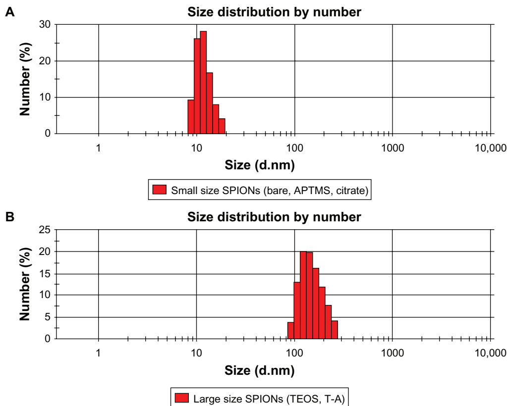
Figure S1 Size distributions of relatively small SPIONs (ie, bare and APTMS- or citrate-coated) ( A ) and large SPIONs (ie, TEOS- or T-A-coated) ( B ) in aqueous solution. Note: The Zetasizer histograms shown in this figure are representative of five independent experiments with almost similar results.
