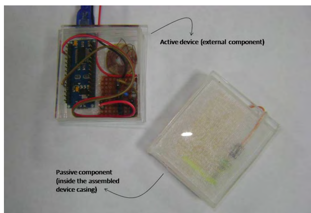
FIGURE 10. Showing the final assembled device with casing, along with the active external RF components, internal RF components are buried inside the device.
