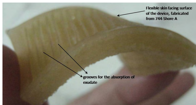
FIGURE 5. Flexible skin facing surface of the device, fabricated from Polyurethane 744, Shore A.
