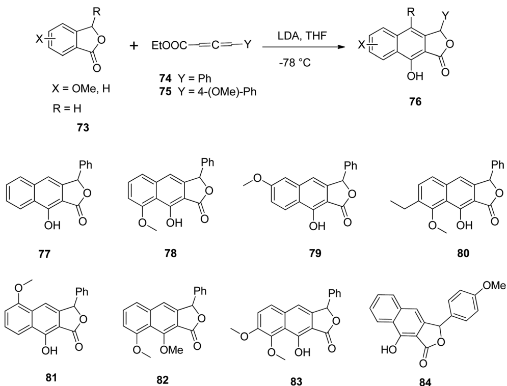
Scheme 10 Synthesis of aryl-naphthalene lactone derivatives. Reagents and conditions: (a) LDA (3 equiv.) and THF, -78 °C to rt, 6–7 h, quenched with 3 M HCl; (b) MeI, \text{K}_2\text{CO}_3 and acetone, room temperature, 4–8 h; (c) crude product, \text{K}_2\text{CO}_3 and acetone, room temperature, 3 days.
