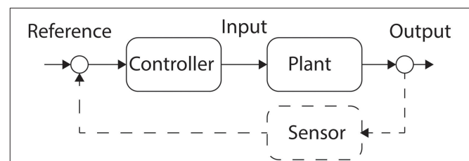
FIGURE 2 | Feedforward and Feedback Control. Feedforward or open-loop control is shown here in the solid line. The controller generates a command that is applied to the system, or Plant. In response to the command the system performs an action at the Output. Closed-loop or feedback control is achieved by the inclusion of the Sensor component, shown here as the dashed line. The Sensor measures the Output enabling the Controller to assess the error and adjust the next Input to the Plant.
