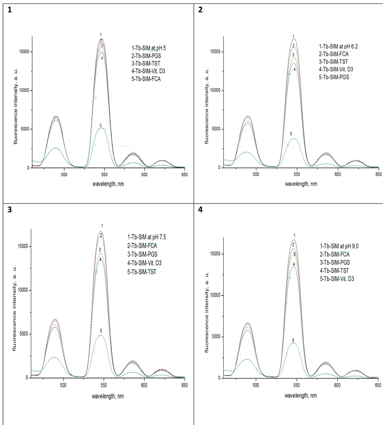
Fig. 6 The luminescence spectra of the complexes Tb-SIM, Tb-SIM-FCA, Tb-SIM-PGS, Tb-SIM-TST and Tb-SIM-Vit-D 3 at \lambda_{ex} = 340 nm and different pHs; (1) 5.0, (2) 6.2, (3) 7.5 and (4) 9.0.
