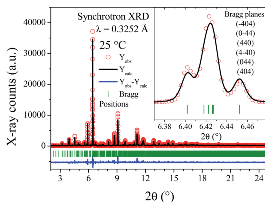
Fig. 3 SXRPRD pattern at room temperature, after the Rietveld refinement in a triclinic lattice. Inset: Detailed view of main reflection, including the planes obtained from the (440) cubic one.
