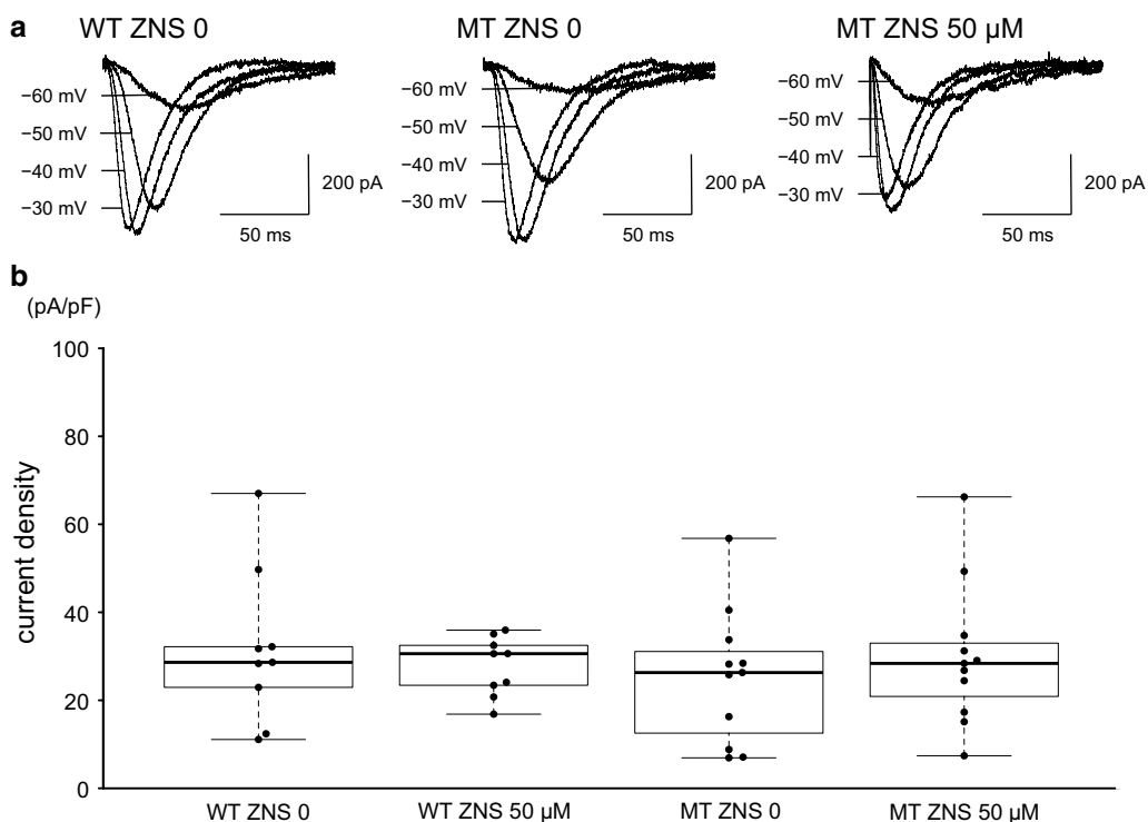
Fig. 1 Effect of ZNS on mutant Ca_v3.1 . a Representative traces of T-type VDCC currents recorded from HEK293T cells expressing WT without ZNS (left), MT without ZNS (middle), or MT with 50 \mu M ZNS (right). WT is wild-type and MT is mutant Ca_v3.1 . b Comparison of Ca^{2+} current density at a holding potential of -30 mV. No significant difference was observed between WT without ZNS and each group (WT with 50 \mu M ZNS, p=0.588 ; MT without ZNS, p=0.355 ; MT with 50 \mu M ZNS, p=0.816 )
