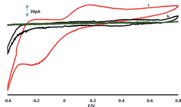
Fig. 4 CVs measured in PBS with a pH of 2.0: (a) GPE, (b) GPE/A and (c) GPE/PtAM.
