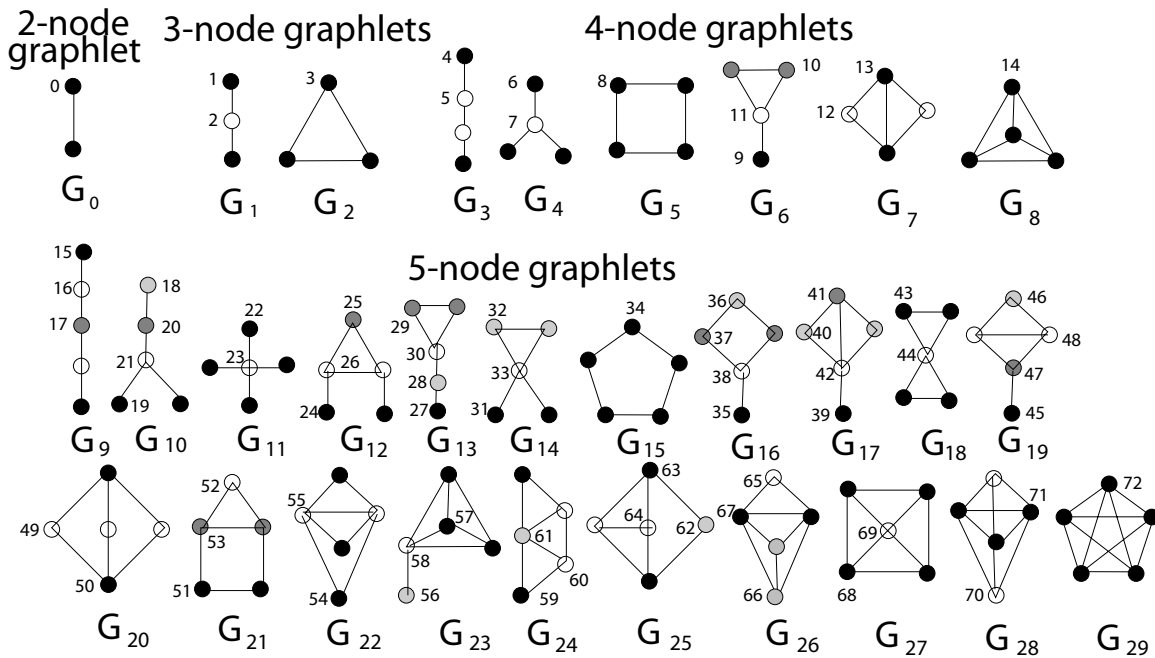
Figure 1. The thirty 2-, 3-, 4-, and 5-node graphlets G_0, G_1, \dots, G_{29} and their automorphism orbits 0, 1, 2, \dots, 72 . In a graphlet G_i , i \in \{0, 1, \dots, 29\} , nodes belonging to the same orbit are of the same shade (Pržulj, 2006).
