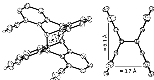
Fig. 3 Different views on the molecular structure of photo-dimer syn-2 in the crystalline state. Displacement ellipsoids are drawn at 50% probability level. Hydrogen atoms, except those of the ethynyl groups, are omitted for clarity. The values shown are averaged distances between the ethynyl protons. For selected bond lengths and angles, see Fig. S19 (ESI).†
