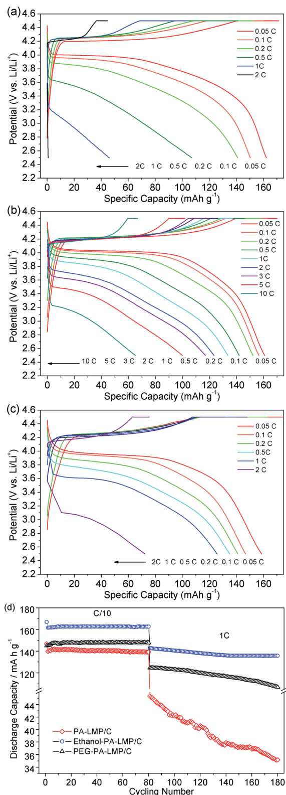
Fig. 7 Charge and discharge profiles of PA-LMP/C (a), ethanol-PA-LMP/C (b), PEG-PA-LMP/C (c) and cycling performances of three \text{LiMnPO}_4/\text{C} composites (d).
