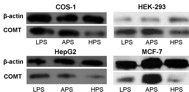
Figure 4. Protein expression levels of COMT constructs that code for three COMT haplotypes in the range of mammalian cell lines. The constructs were transiently transfected into indicated cell lines and its protein expression were analyzed via western blotting. Top band: \beta -actin. Lower band: COMT. Cell lines: COS-1 monkey kidney cells, HEK-293 human embryonic kidney cells, HepG2 human liver cells, and MCF-7 human breast cells. Among these cell lines, APS protein expression is equivalent or higher than LPS, while HPS exhibits significantly lower levels compared to the two haplotypes.
