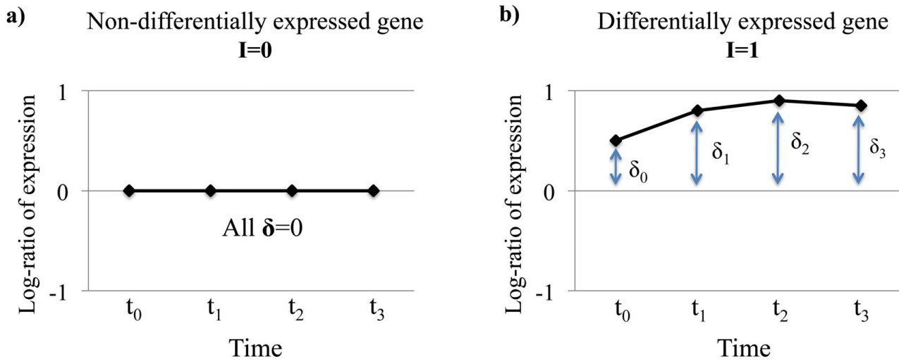
Figure 1 Time-course expression profiles of two illustrative genes. Log-ratio of expression between two treatment groups for a) a gene without differential expression, and b) an illustrative differentially expressed gene. I is an indicator of differential expression. \delta represents the log-fold change at the four time points.
