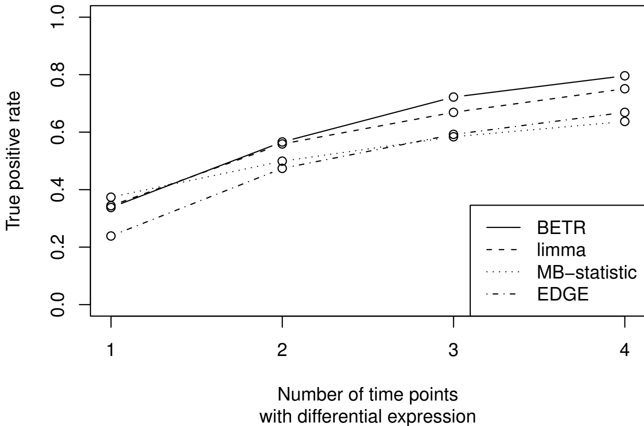
Figure 3 Performance assessment: True positive rate vs. number of time points with differential expression. True positive rate as a function of the number of the four time points with differential expression. The significance cutoff is chosen to maintain a false positive rate of 5%.
