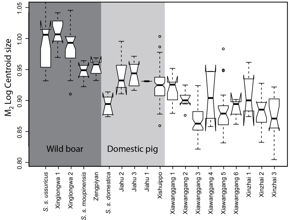
Fig 2. Notched boxplot of the M_2 Log transformed centroid size for all samples. The box represents 50% of the variation around the median (horizontal black line); the brackets represent the minimum and maximum. Notches represent a 95% interval confidence of the median.
