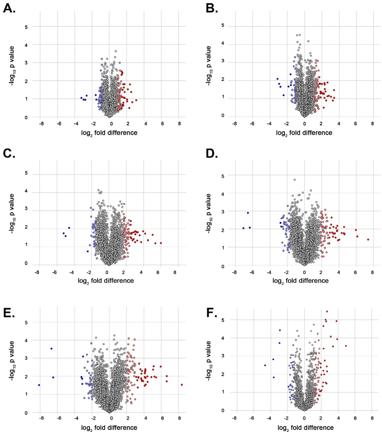
FIGURE 2. Volcano plots illustrating the differentially expressed proteins in the mouse lens at different developmental time points. The proteins identified in all three TMT datasets (i.e., 3155) were examined to classify significantly upregulated and downregulated proteins, compared with their respective expression levels at embryonic day 15 (E15). Volcano plots showing differentially expressed proteins at (A) embryonic day 18 (E18), (B) postnatal day 0 (P0), (C) postnatal day 3 (P3), (D) postnatal day 6 (P6), and (E) postnatal day 9 (P9) when compared with the earliest time point E15, and (F) the differential expression of proteins between embryonic time points (E15 and E18) and postnatal time points (P0, P3, P6, and P9). The x-axis corresponds to the \log_2 fold change value, and the y-axis displays the -\log_{10} P value. Proteins that are significantly upregulated ( \geq +2 standard deviations) are highlighted in red and light red, and those with significant downregulation ( \geq -2 standard deviations) are highlighted in blue and light blue.
