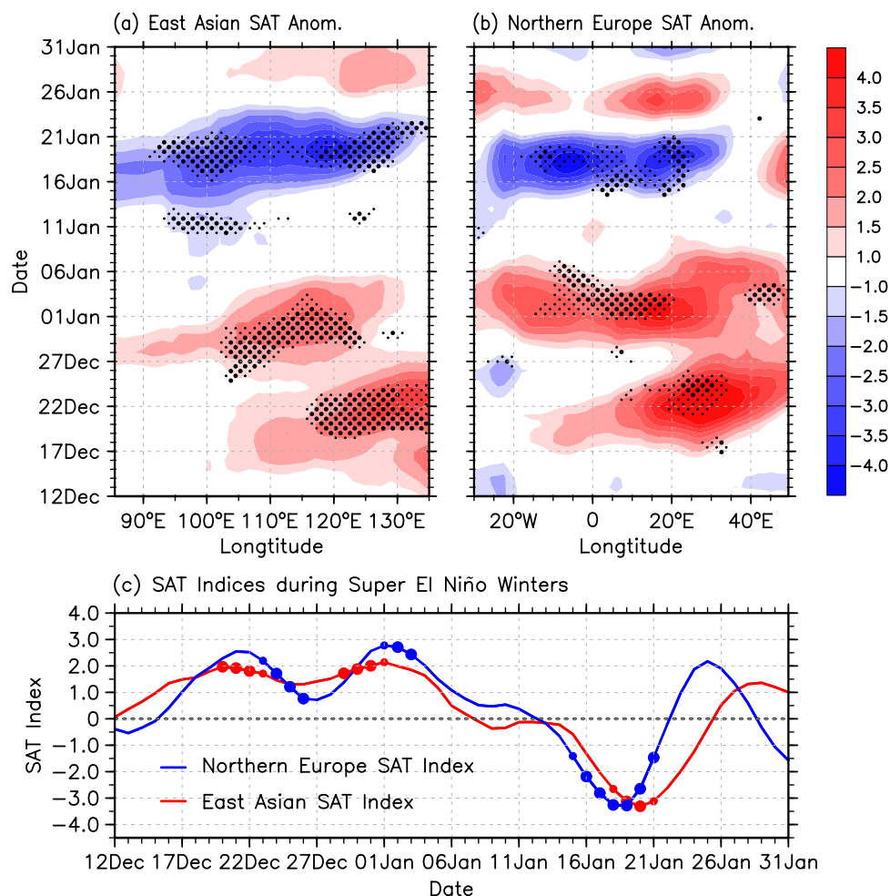
Figure 2. Regional wintertime SAT responses to super El Niño on the sub-seasonal timescale. Composite time-longitude sub-seasonal variation of (a) East Asian ( 25^{\circ} – 55^{\circ} N average) and (b) Northern Europe ( 60^{\circ} – 80^{\circ} N average) SAT anomalies ( ^{\circ} C) for super El Niño winters (1982/83, 1997/98, and 2015/16). Small and big black dots indicate the anomalies above the 90 and 95% confidence levels, respectively. (c) Composite sub-seasonal variability of the East Asian (red line) and Northern Europe (blue line) SAT indices ( ^{\circ} C) for super El Niño winters. Small and big dots represent the corresponding SAT anomalies above the 90 and 95% confidence levels, respectively. The figure was generated with the NCAR Command Language (Version 6.3.0) [Software] (2015). Boulder, Colorado: UCAR/NCAR/CISL/TDD. http://www.ncl.ucar.edu/ .
