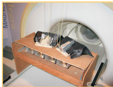
Figure 1. Device for passive movement stimulation. Picture of the MR compatible device for passive motor stimulation of the index- and middle-fingers of the left and right hands.
