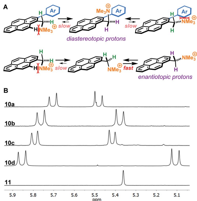
Fig. 3 Differences in benzylic protons between pyrene cations in this study. (A) Rotamers along the C sp^2 –C sp^3 bond of arylated ( 10a–d ) and non-arylated ( 11 ) pyrene cations. (B) ^1\text{H-NMR} signals of benzylic protons in compounds 10a–d and 11 in methanol- d_4 . The diastereotopic benzylic protons of arylated compounds 10a–d indicate that the ammonium group is locked pointing away off the pyrene ring plane. The second set of benzylic protons of compound 10c appear outside the shown range. See ESI† for full spectra.
