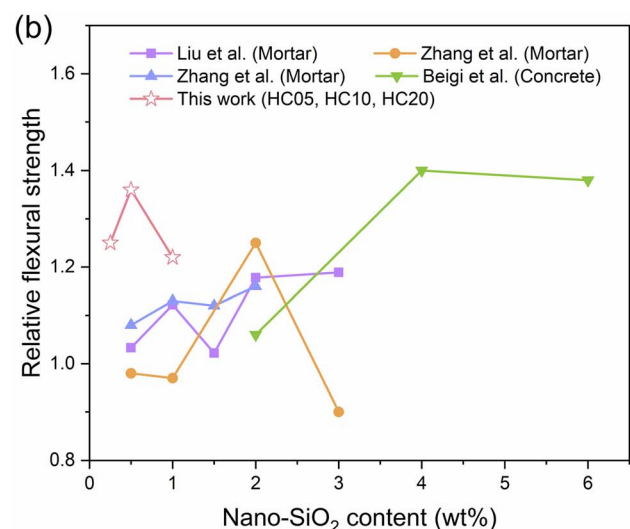
Fig. 15 Comparison results of reinforcement effects on cement materials with addition of CNTs 54–57 (a) and nano-SiO 2 (ref. 23, 24, 40 and 58) (b). Relative flexural strength was calculated with the plain samples as references in different literature.
