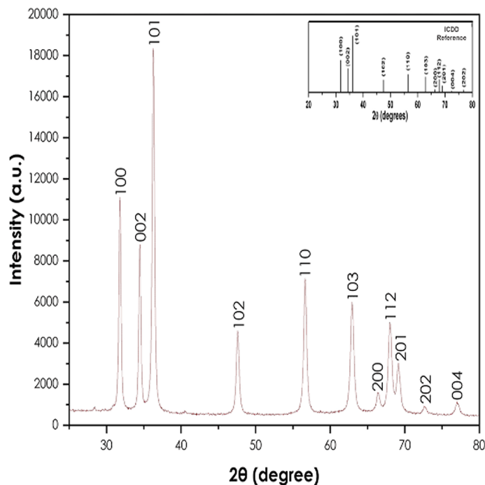
Figure 4. X-ray diffraction pattern of ZnO nanoparticles.
