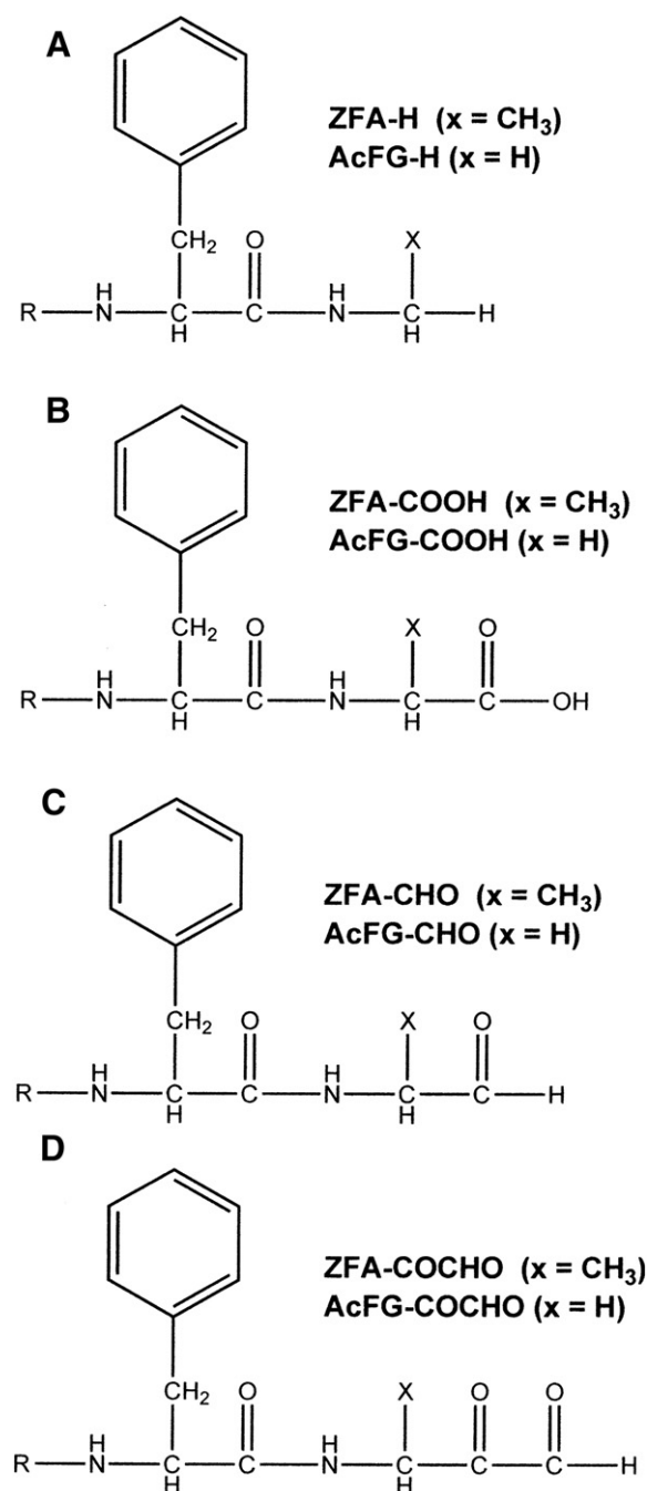
Scheme 1. Structures of inhibitors. a a R and X are either Z and CH 3 – for ZFA (Z-Phe-Ala–) or Ac and H for AcFG (Ac-Phe-Gly–).
