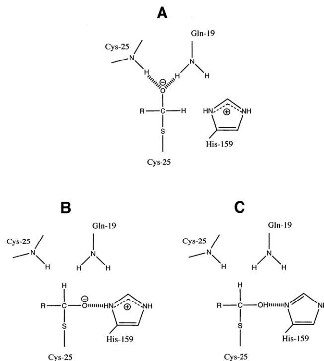
Scheme 4. Thiohemiacetals formed when aldehyde inhibitors inhibit papain and enzymes of the papain family.
