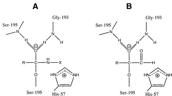
Scheme 5. Comparison of the structures of the catalytic tetrahedral intermediate formed with peptide substrates and the hemiketal formed when glyoxal inhibitors react with chymotrypsin.
