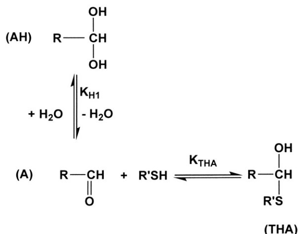
Scheme 3. Minimal scheme for thiohemiacetal formation with N-acetyl-L-cysteine.
