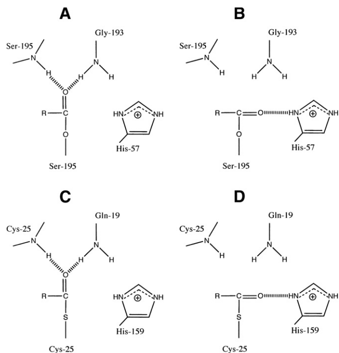
Scheme 6. Structures of the acyl intermediates formed with the serine and cysteine protease.
