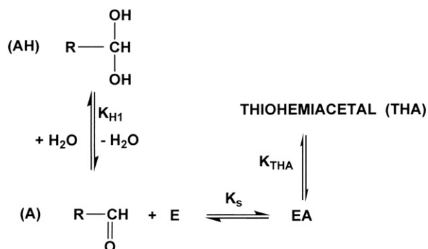
Scheme 2. Minimal scheme for thiohemiacetal formation by the cysteine proteases.
