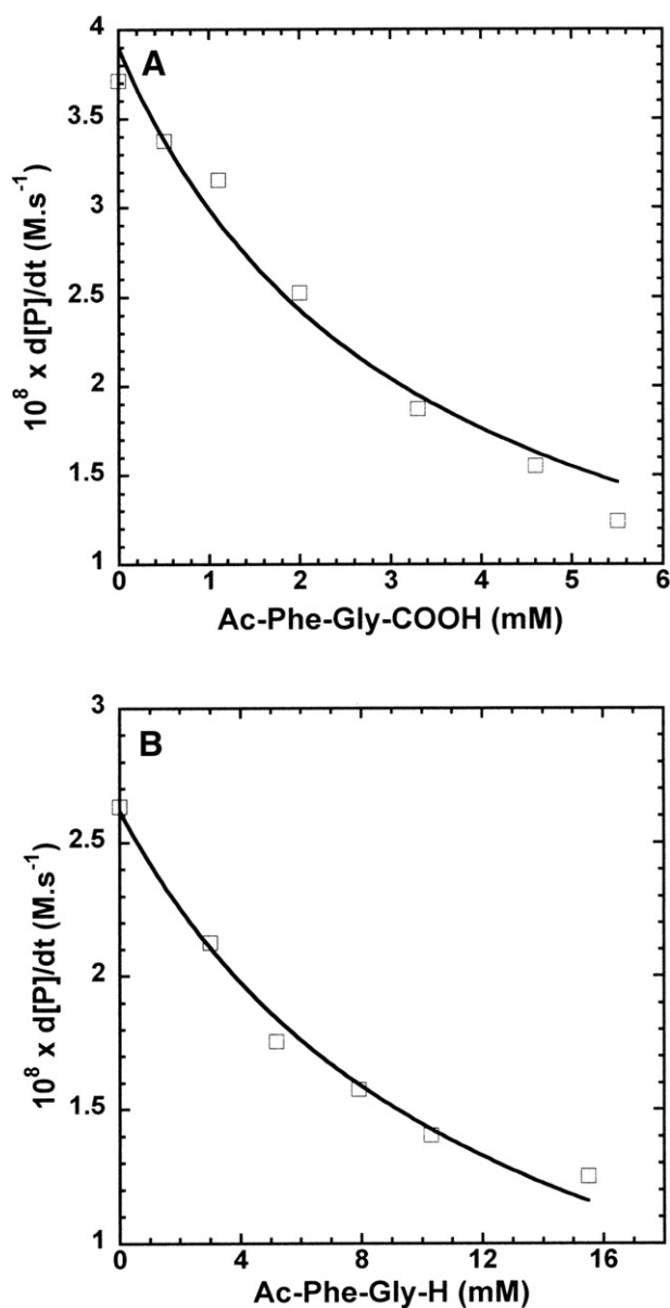
Fig. 1. Inhibition of the papain catalysed hydrolysis of \alpha -N-benzoyl-L-arginine-p-nitroanilide by Ac-Phe-Gly-H and Ac-Phe-Gly-COOH. All samples contained 1.67% (v/v) dimethyl sulfoxide and 0.1 M potassium phosphate buffer at pH 7.0. (A) For inhibition by Ac-Phe-Gly-COOH the concentrations of \alpha -N-benzoyl-L-arginine-p-nitroanilide and active papain were 0.25 mM and 0.6 \mu M respectively. The solid line was calculated using the equation d[P]/dt = ((k_{cat}/K_M)[E][S] K_i)/([I] + K_i) and the fitted values of 260 \pm 10 \text{ M}^{-1} \text{ s}^{-1} and 3.30 \pm 0.42 \text{ mM} for k_{cat}/K_M and K_i respectively. (B) Inhibition by Ac-Phe-Gly-H was measured in the same way with substrate and active enzyme concentrations of 0.23 mM and 0.48 \mu M respectively. The solid line was calculated as in (A) using the fitted values of 237 \pm 5 \text{ M}^{-1} \text{ s}^{-1} and 12.3 \pm 1.0 \text{ mM} for k_{cat}/K_M and K_i respectively. All the errors quoted in this figure legend are standard errors obtained on fitting the experimental data. Experimental data were obtained at 25 °C.
