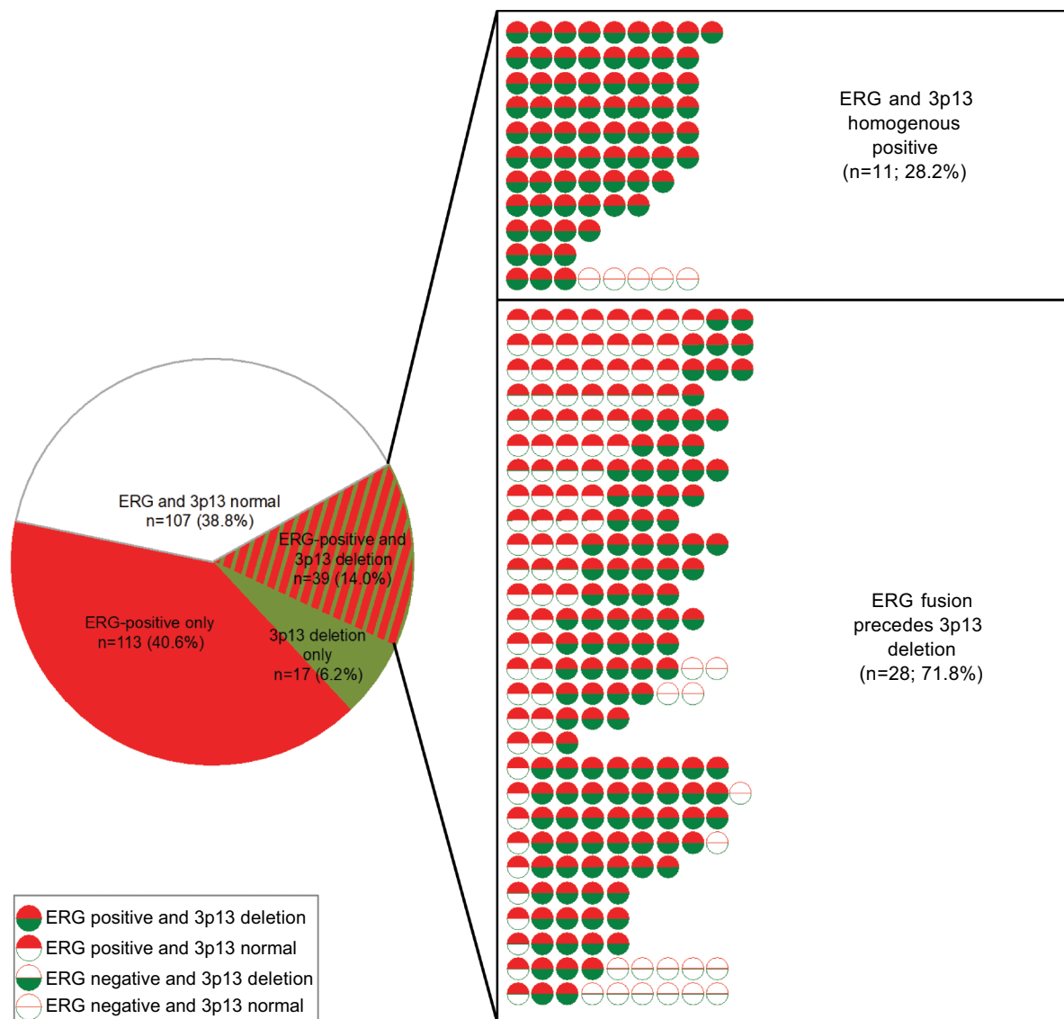
Figure 4 Association between 3p13 deletion and ERG expression at the cancer level.
