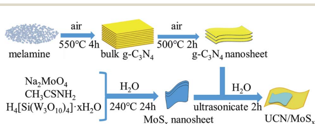
Fig. 1 Schematic diagram for the synthesis of MoS x /UCN composite.
