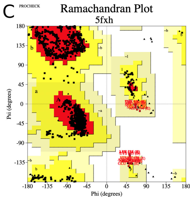
Figure S5. Ramachandran plots. (A) The di-heteromeric GluN1a/GluN2A homology model selected for this study. (B) The di-heteromeric template used PDB identifier 4PE5 (GluN1/GluN2B). (C) The second di-heteromeric template used PDB identifier 5FXH (GluN1/GluN2B) consisting of only backbone atoms.
