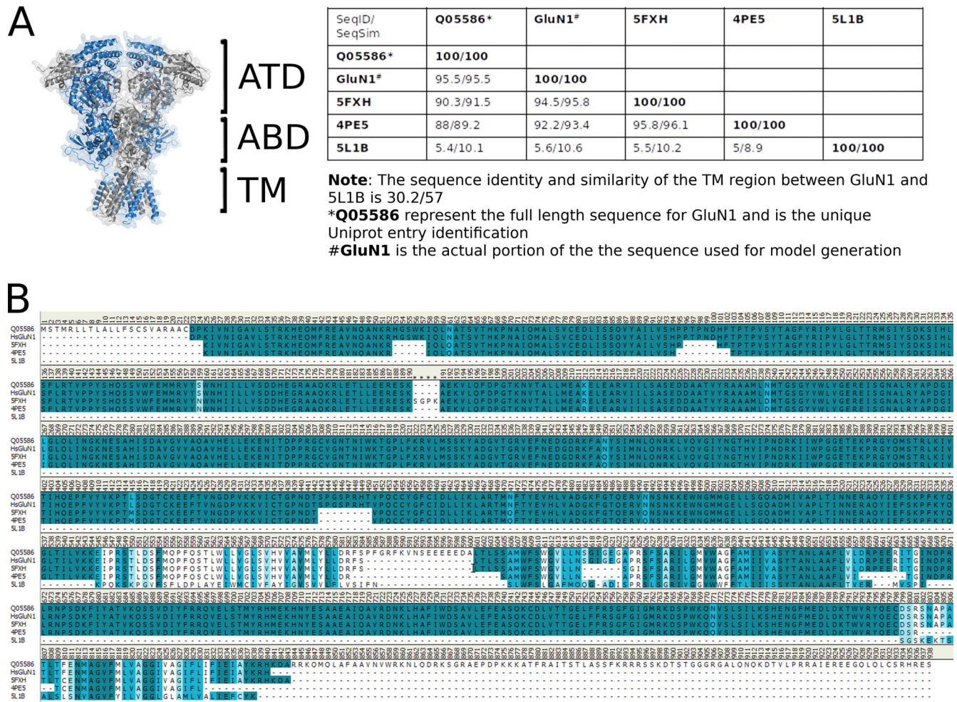
Figure S3. Sequence alignments used for homology model building. (A) An image of a full-length di-heterotetramer GluN1 (gray)/GluN2A (blue) NMDA structure. The table provides the sequence identity (SeqID) and sequence similarity (SeqSim) of the template and target sequences used for GluN1. (B) The sequence alignment used for GluN1 during model building.
