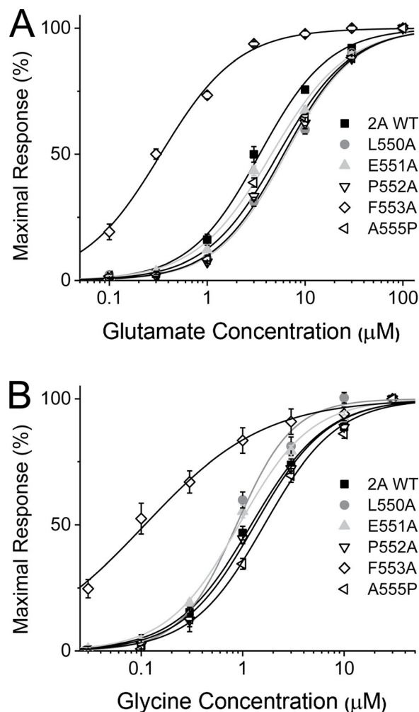
Figure 2. Mutations in the GluN2 pre-M1 helix shift glutamate and glycine potency. Steady-state concentration–response curves for glutamate in the presence of 100 \mu\text{M} glycine (A) and glycine in the presence of 100 \mu\text{M} glutamate (B). The Hill equation was fitted to the composite data for GluN2A WT and GluN2A-L550A, GluN2A-E551A, GluN2A-P552A, GluN2A-F553A, and GluN2A-A555P expressed with WT GluN1. GluN2A-F553A shifted glutamate potency \sim 11 -fold ( EC_{50} from 3.6 \mu\text{M} to 0.34 \mu\text{M} ) and glycine potency \sim 18 -fold ( EC_{50} from 1.4 \mu\text{M} to 0.077 \mu\text{M} ). Fitted EC_{50} values for all mutants can be found in Table 2.
