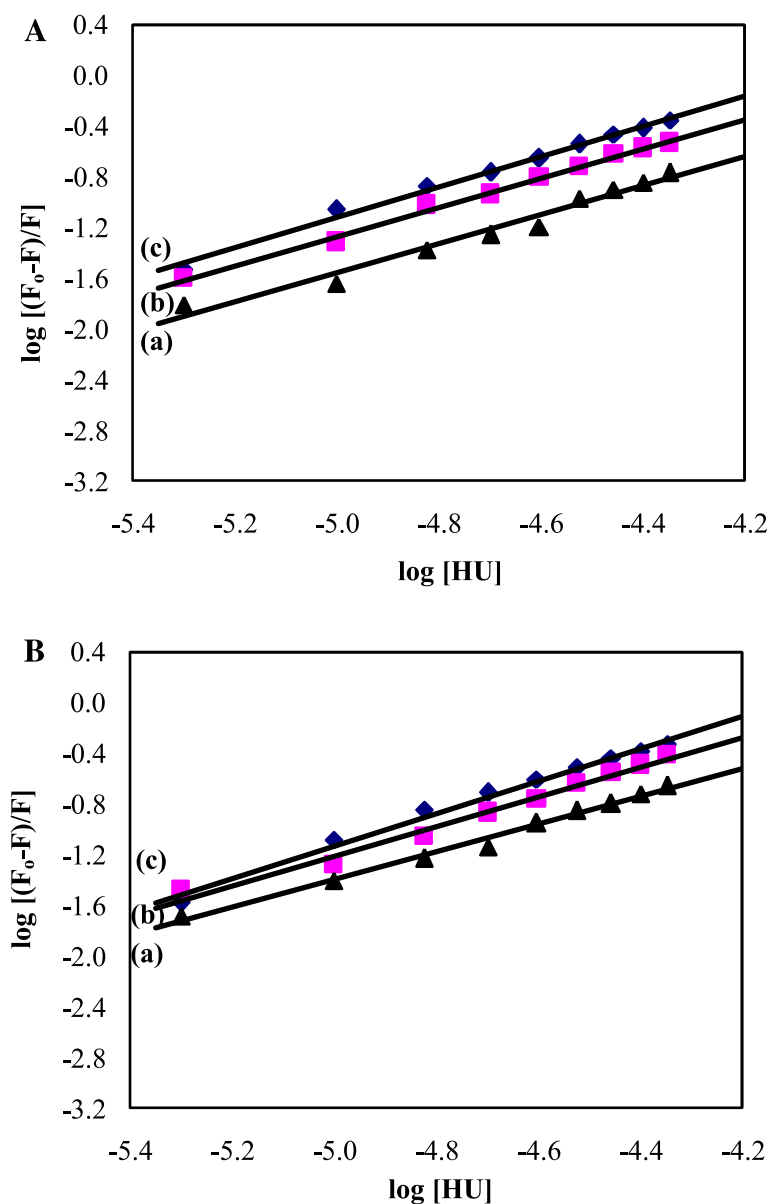
Figure 4 The plot of \log of BSA and HSA. A. The plot of \log (F_0-F)/F vs \log [Q] for quenching of BSA by HU at 288 K (a), 298 K (b) and 308 K (c). B. The plot of \log (F_0-F)/F vs \log [Q] for quenching of HSA by HU at 288 K (a), 298 K (b) and 308 K (c).
