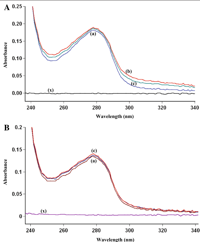
Figure 6 Absorbance spectra of BSA and HSA. A. Absorbance spectra of BSA, HU and HU-BSA system. BSA concentration was 5 \mu\text{M} (a). HU concentration for HU-BSA system was at 5 \mu\text{M} (b) and 10 \mu\text{M} (c). (x) is the concentration of 5 \mu\text{M} HU. B. Absorbance spectra of HSA, HU and HU-HSA system. HSA concentration was 5 \mu\text{M} (a). HU concentration for HU-HSA system was at 5 \mu\text{M} (b) and 10 \mu\text{M} (c). (x) is the concentration of 5 \mu\text{M} HU.
