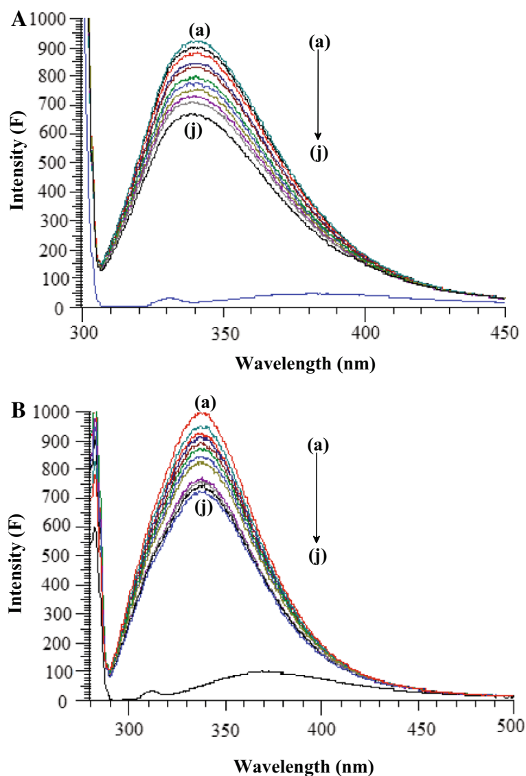
Figure 2 Fluorescence spectra of BSA and HSA. A. Fluorescence spectra of BSA (5 μM) in presence of HU: (a) 0 μM, (b) 5 μM, (c) 10 μM, (d) 15 μM, (e) 20 μM, (f) 25 μM, (g) 30 μM, (h) 35 μM, (i) 40 μM, (j) 45 μM. B. Fluorescence spectra of HSA (5 μM) in presence of HU: (a) 0 μM, (b) 5 μM, (c) 10 μM, (d) 15 μM, (e) 20 μM, (f) 25 μM, (g) 30 μM, (h) 35 μM, (i) 40 μM, (j) 45 μM.
