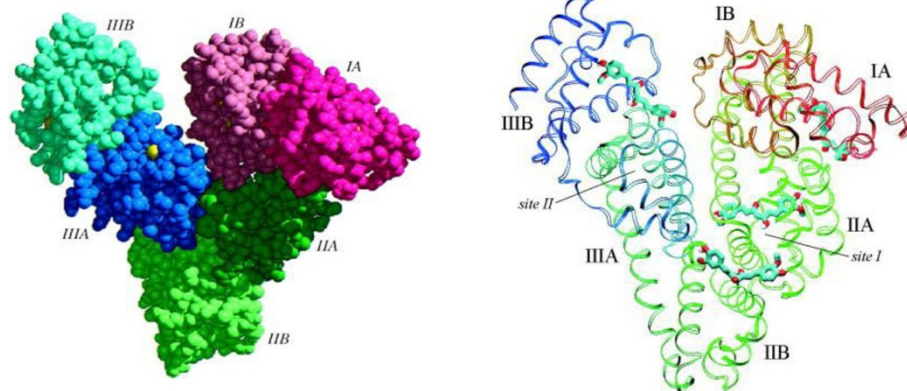
Figure 1 Structure of BSA and HSA.
