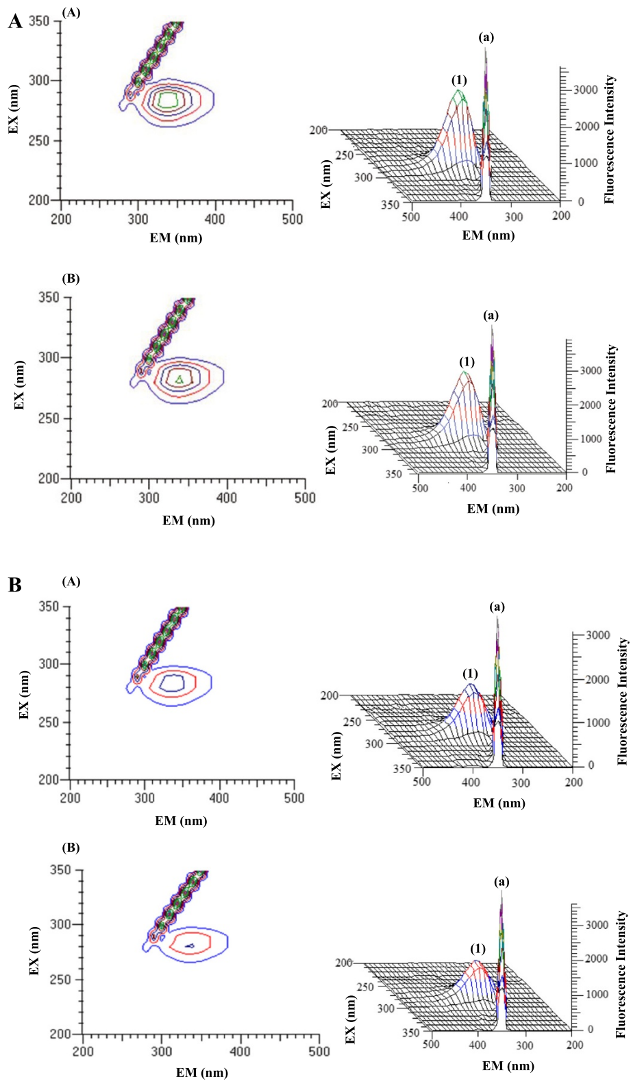
Figure 9 The 3-D fluorescence spectra of BSA and HSA. A. The 3-D fluorescence spectra and corresponding contour diagrams of BSA ( A ) and BSA-HU ( B ). The concentration of protein was 5 \mu\text{M} and that of HU was 20 \mu\text{M} . B. The 3-D fluorescence spectra and corresponding contour diagrams of HSA ( A ) and HSA-HU ( B ). The concentration of protein was 5 \mu\text{M} and that of HU was 20 \mu\text{M} .
