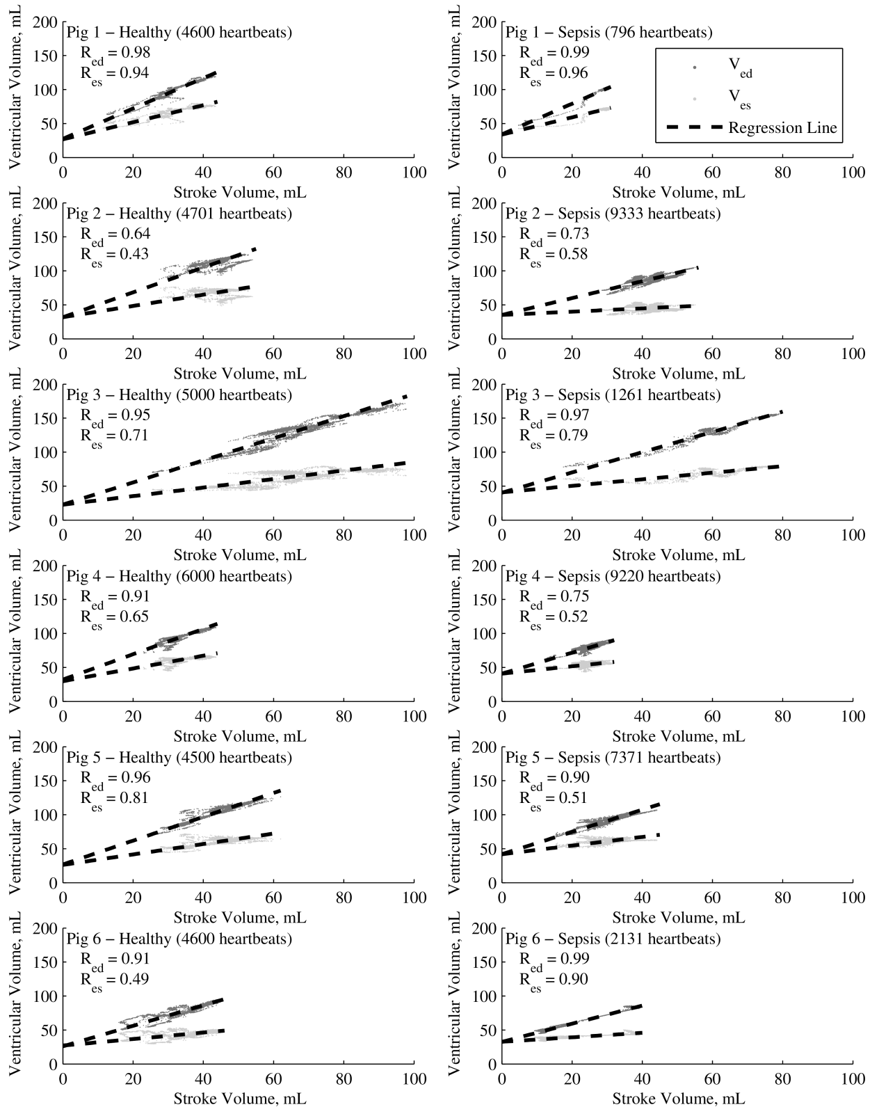
Fig 3. Pre- (left) and post- (right) endotoxin infusion SV- V_{ed} , SV- V_{es} curves and regression lines for each pig. Number of heartbeats and Pearson's Correlation Coefficients ( R ) presented in figure.
