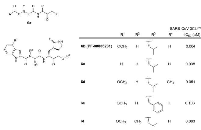
Figure 6. Structures from WO 2005/113580. (a) general scaffold; (b–f) exemplified structures.
