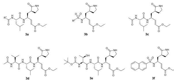
Figure 3. Structures from US 2006/0014821. (a, b) general scaffolds; (c–f) exemplified structures.
