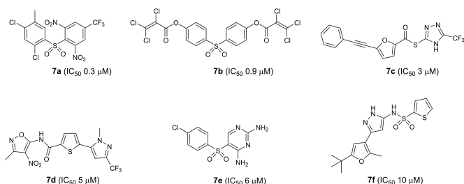
Figure 7. Six most potent SARS-CoV 3CL pro inhibitors reported in US 2006/0019967.
