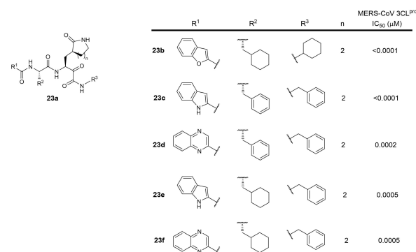
Figure 23. Structures from WO 2020/030143. (a) general scaffold; (b–f) most potent exemplified MERS-CoV 3CL pro inhibitors.
