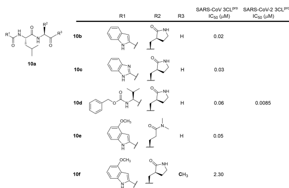
Figure 10. Structures from WO 2006/061714. (a) general scaffold; (b–f) exemplified structures.
