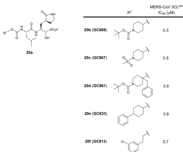
Figure 20. Structures from WO 2017/222935. (a) general scaffold; (b–f) exemplified structures.
