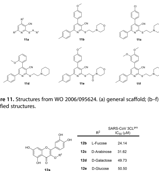
Figure 11. Structures from WO 2006/095624. (a) general scaffold; (b–f) exemplified structures.
