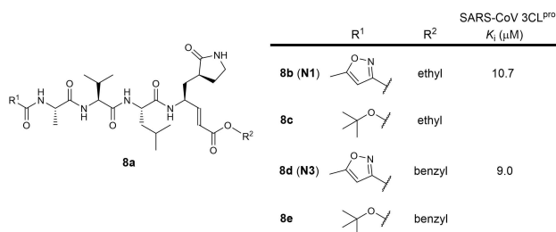
Figure 8. Structures from WO 2006/061714. (a) general scaffold; (b–e) exemplified structures.
