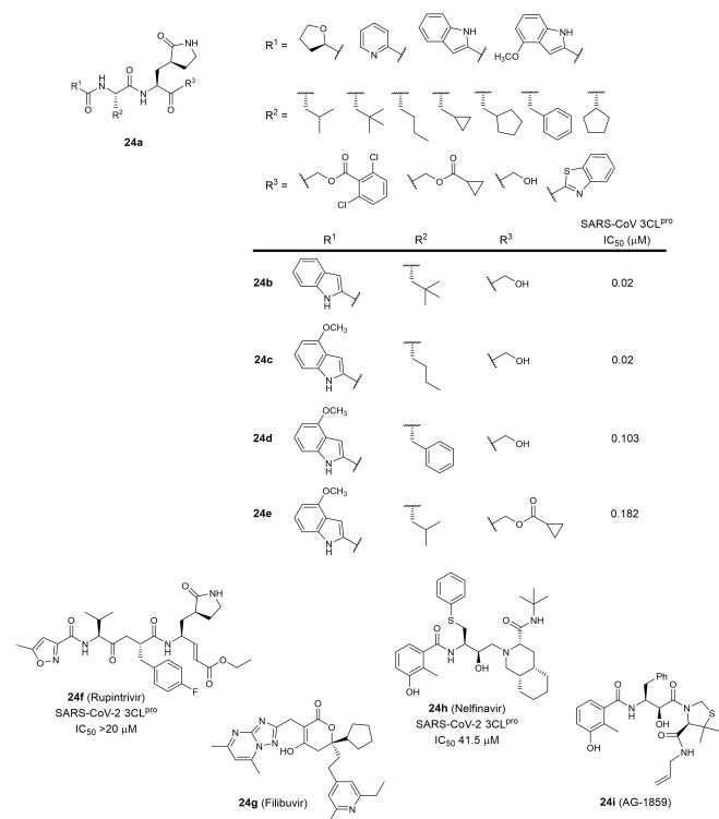
Figure 24. Structures from WO 2021/176369. (a) peptidomimetic general scaffold; (b–i) exemplified inhibitors.
