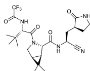
Figure 25. Structure of PF-07321332.
