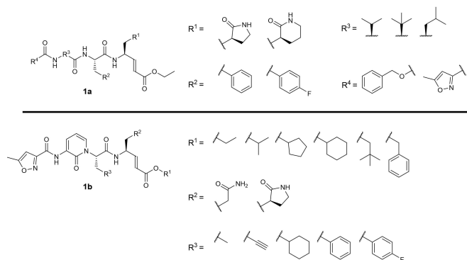
Figure 1. General scaffolds from WO 2004/093860.
