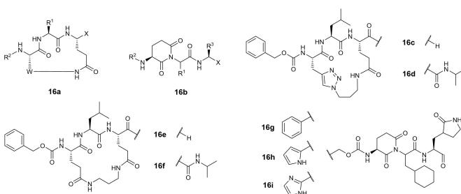
Figure 16. Structures from WO 2013/166319. (a, b) general scaffolds; (c–i) exemplified structures.
