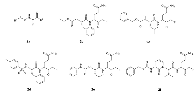
Figure 2. Structures from WO 2004/101742. (a) general scaffold; (b–f) exemplified structures.
