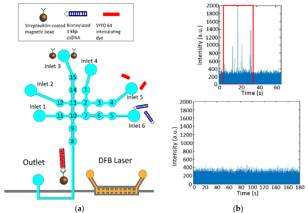
Figure 5. (a) Non-specific biomarker detection. Streptavidin-coated magnetic beads with capture probes are loaded into inlet 3 while the SYTO 64 intercalating dye and biotinylated 1kbp dsDNA are introduced into inlets 5 and 6, respectively. Inlets 1, 2, and 4 were loaded with 1xPBS buffer. Samples are brought together into the central mixing valves (13, 2, 7, 10) where they are mixed and incubated for the proper construct to be formed. Beads with captured fluorescently stained targets are pulled down with a magnet while excess targets and unconjugated probes are washed using buffer. The magnet is then removed, and the complete bead constructs are pushed to the detection region. (b) Fluorescence time domain trace illustrating peaks observed from fluorescently stained bead constructs (top). Control trace done in the absence of dsDNA targets illustrating no peaks above the noise floor (bottom).
