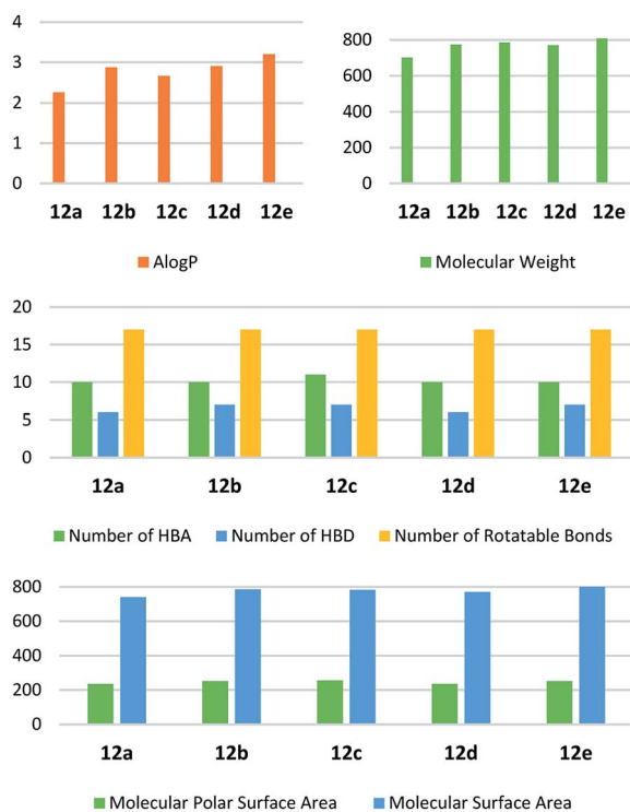
Fig. 2 Physicochemical properties in bar charts: calculated A log P , molecular weight (Da), number of HBD and HBA, number of rotatable bonds, molecular surface area ( \text{\AA}^2 ), and molecular polar surface area ( \text{\AA}^2 ).
