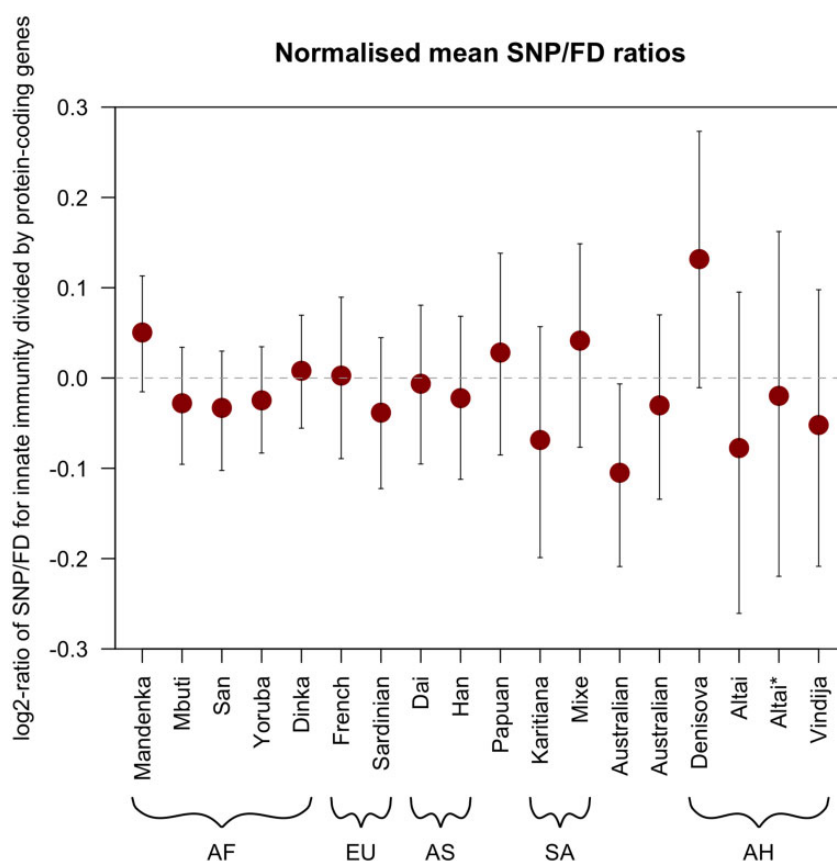
Fig. 2. —Normalized mean SNP/FD ratios ( \log_2 ) for all 17 individuals in the full set of innate immune-related genes ( N = 1,548 ). Error bars give 95% confidence intervals calculated by bootstrapping ( B = 5,000 ). AF, Africa; EU, European; AS, Asian; SA, South American; AH, Archaic Humans. Dashed line gives expected value if the mean values for innate immunity genes and autosomal protein-coding background genes were equal.
