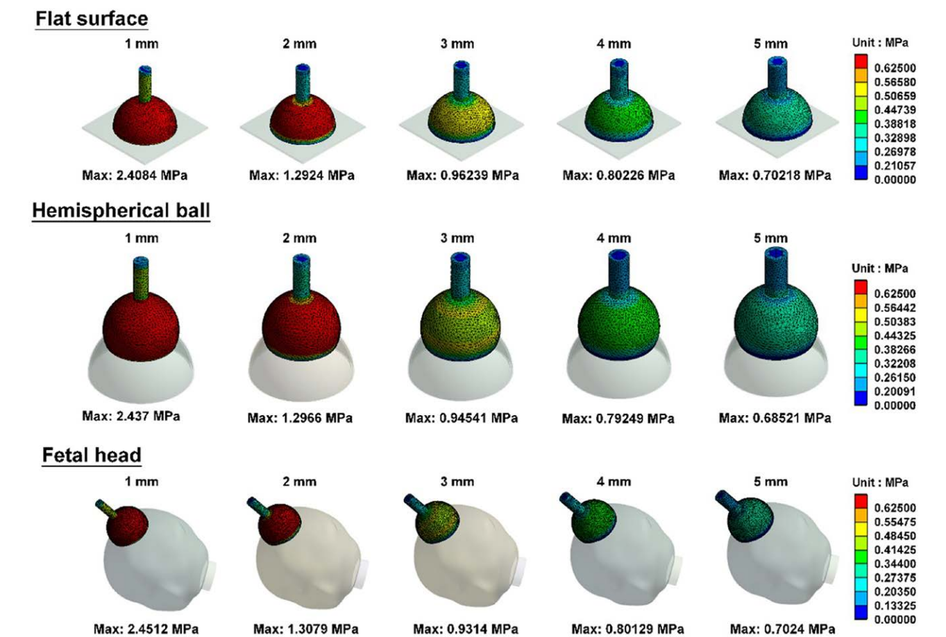
Fig. 4 The von Mises stress distributions of the vacuum extractors when various thicknesses of the vacuum extractors are applied to different surface areas.
