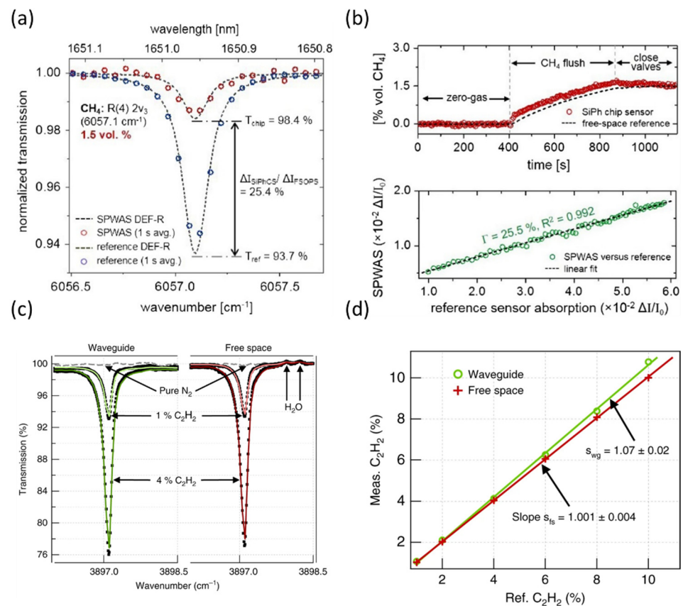
Figure 3. Experimental demonstration of gas detection by WIRAS. (a) The spectrum of the methane R(4)2ν 3 line measured by the waveguide-based integrated spectrometer design by Zhang et al. [157]. The Voigt spectral fit for 1.5% methane concentration is shown in red, together with the experimental data. (b) Upper plot: experimentally measured methane concentration before and after flushing the chamber with methane. Lower plot: correlation between the absorption measured with the waveguide device and a free-space reference beam, indicating \Gamma = 25.5\% in the waveguide (reproduced with permission from reference [157]). (c) Comparison of experimental absorption spectra for 4% and 1% acetylene measured using a free-standing tantala waveguide and a free space beam of identical path length, reproduced from Vlk et al. [69]. (d) Correlation of the measured concentration to the reference concentration of data in (c). The slope gives \Gamma = 107\% (reproduced with permission under a Creative Commons Attribution 4.0 International License. http://creativecommons.org/licenses/by/4.0/ assessed on 9th September 2021).
