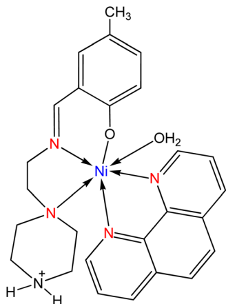
Fig. 31 Water-soluble mixed-ligand nickel(II) complexes.
