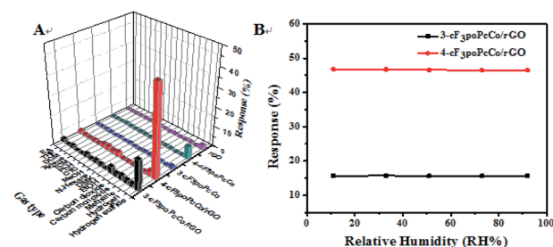
Fig. 3 (A) Response of RPCos, rGO and RPcCo/rGO hybrid-based sensors to 1 ppm of H 2 S and 1000 ppm of various other gases, respectively. (B) Response of the cF 3 poPcCo/rGO hybrid-based sensors to 1 ppm H 2 S at different relative humidities at 25 °C.
