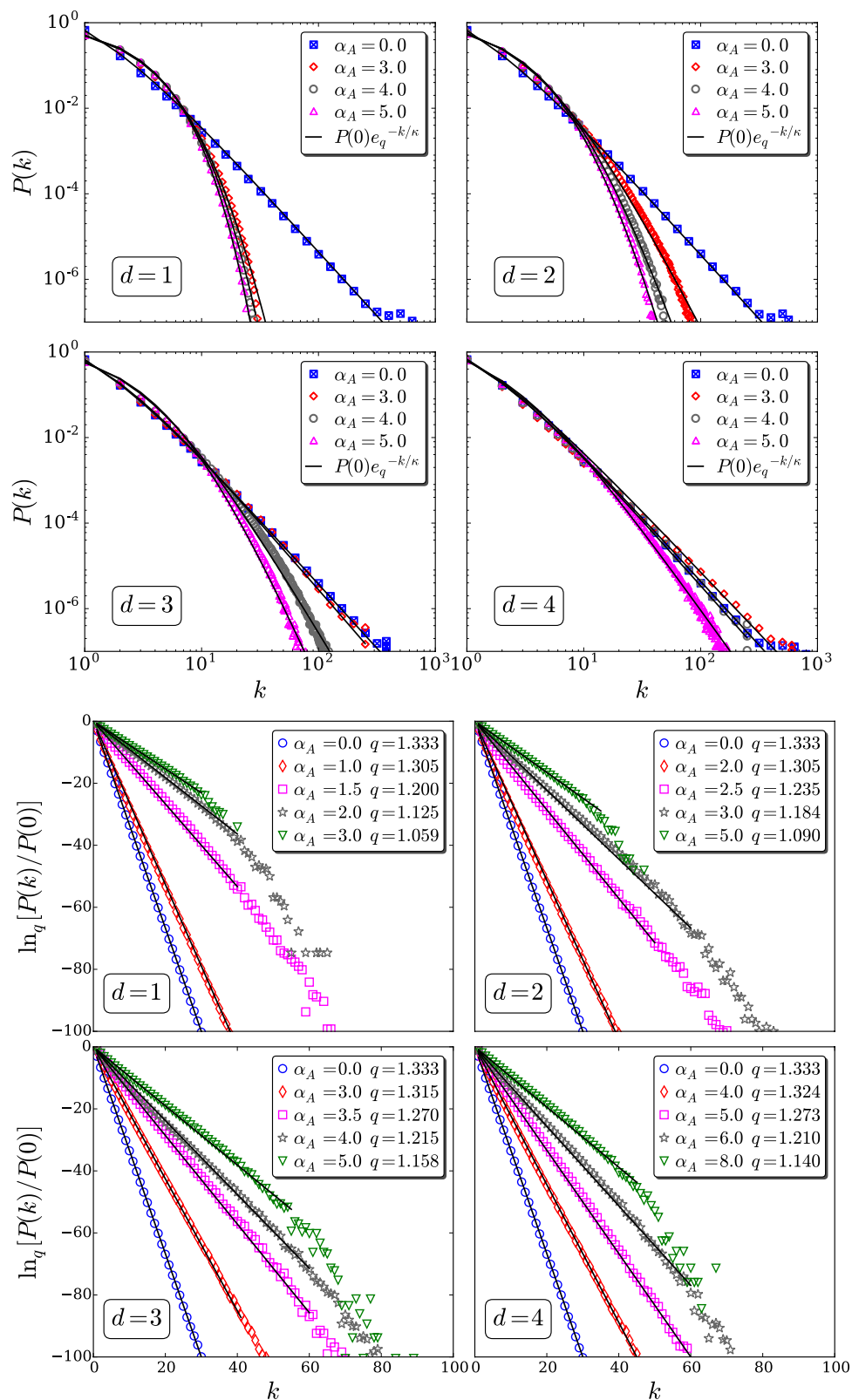
Figure 4. Fittings of the d=1, 2, 3, 4 connectivity distributions with the function P(k) = P(0)e_q^{-k/\alpha} , where e_q^z \equiv [1 + (1 - q)z]^{1/(1-q)} . The data are those of Fig. 3. Top : log-log representation. Bottom : \ln_q[P(k)/P(0)] versus k representation. Notice that straight lines in a \ln_q -linear representation univocally determine the q -exponential function. The fitting parameters are exhibited in Fig. 5. The numerical failure, at large enough values of k , with regard to straight lines are finite-size effects that gradually disappear when we approach the thermodynamic limit N \rightarrow \infty . Logarithmic binning was used whenever convenient.
