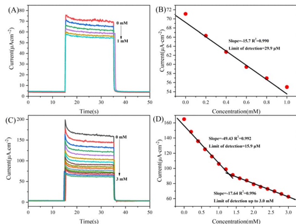
Fig. 7 Photoelectrochemical responses with different concentrations of glucose of ZnO (A) and Vo-ZnO/ZnS (C) and the calibration curves between the photocurrent and the concentration of glucose of ZnO (B) and Vo-ZnO/ZnS (D).
