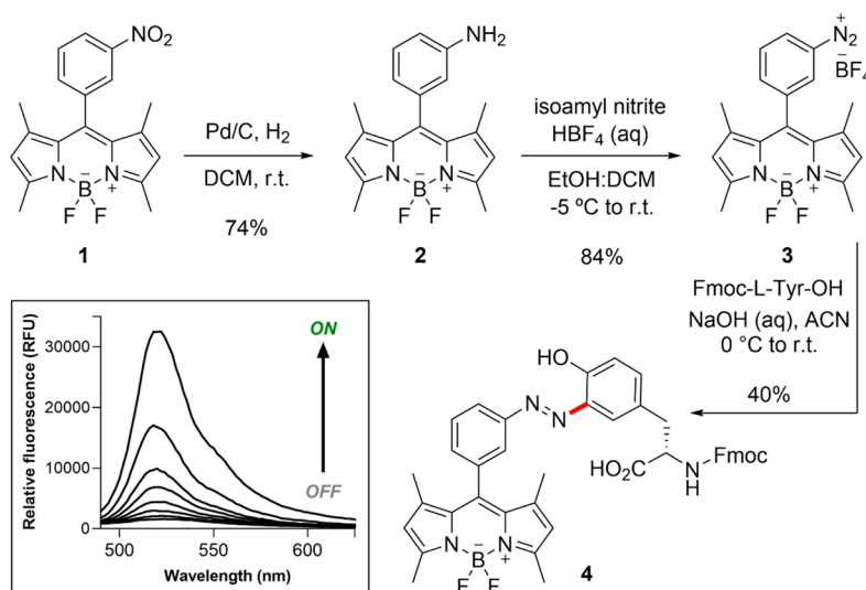
Figure 2. Synthesis of diazonium BODIPY and Tyr-BODIPY adducts. Synthetic scheme for the preparation of Tyr-BODIPY amino acids. (Left) Representative fluorescence spectra of compound 4 (25 \mu M) in phosphate buffer saline (PBS) and after incubation with increasing concentrations of phosphatidylcholine liposome suspensions (from 3.75 to 0.004 mg mL -1 in PBS (excitation: 450 nm).
