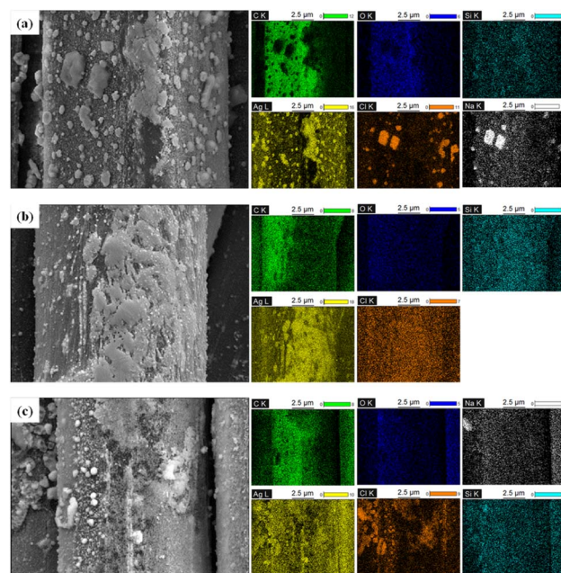
Fig. 2 FE-SEM images ( \times 10\ 000 ) and EDX mapping images of grains on the conductive knitted fabrics after exposure to the perspiration: (a) C1; (b) C2; (c) C3.
