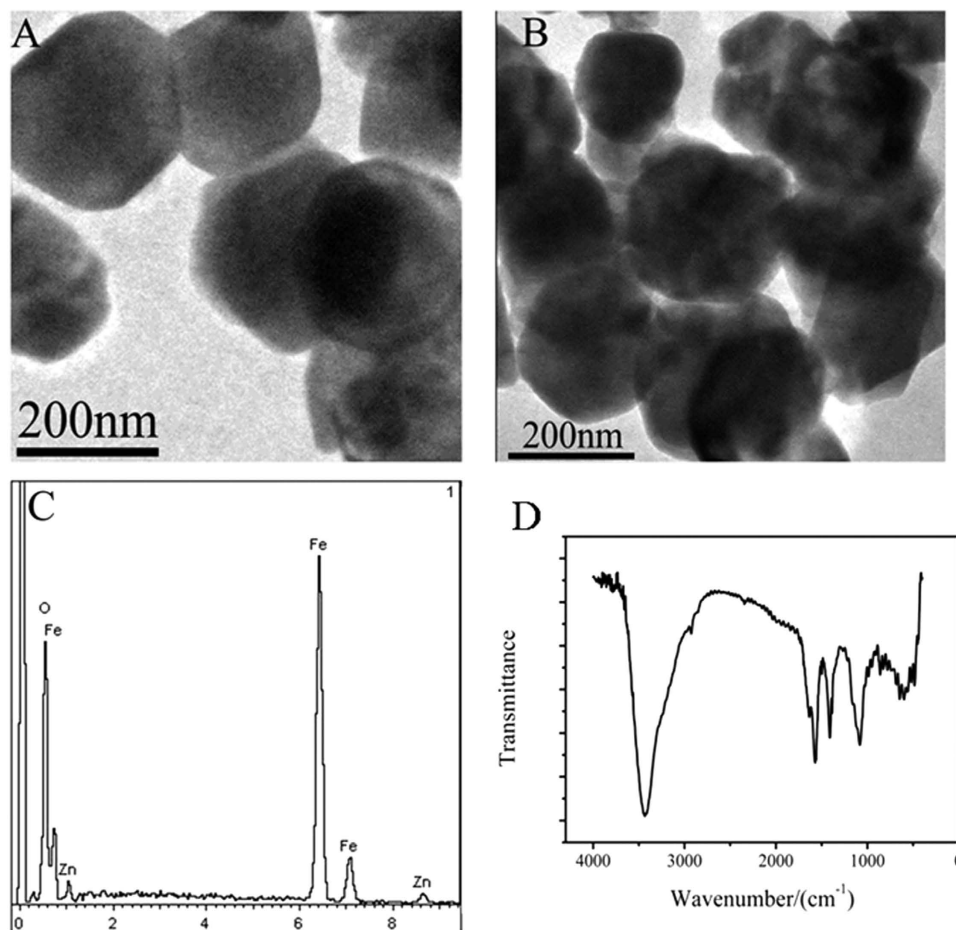
Figure 2. TEM images of \text{Fe}_3\text{O}_4 (A) and \text{Fe}_3\text{O}_4@\text{ZnO} (B); the EDS spectrum of \text{Fe}_3\text{O}_4@\text{ZnO} (C); IR spectra of \text{Fe}_3\text{O}_4@\text{ZnO}@L\text{-Cys} (D).
