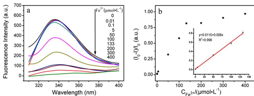
Figure 4. (a) Emission spectra of Fe_3O_4@ZnO@L-Cys in the presence of increasing amounts of Fe^{3+} at room temperature; (b) The curve of fluorescence intensity at 337 nm vs. Fe^{3+} .
