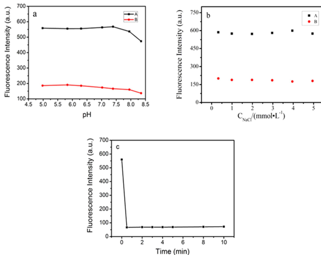
Figure 3. (a) Fluorescence intensity of our proposed nanosensor in the absence (A) and presence (B) of Fe^{3+} at different pH; (b) The effect of ionic strength on fluorescence intensity in the absence (A) and presence (B) of Fe^{3+} ; (c) Time course of the fluorescence response of Fe_3O_4@ZnO@L-Cys in the presence of Fe^{3+} ( 200 \mu mol L^{-1} ). The fluorescence intensity was recorded at 337 nm, with an excitation at 290 nm at room temperature.
