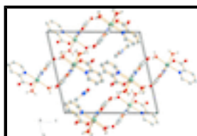
Fig. 2. A packing diagram for the title complex. H-atoms not involved in H-bonds are omitted for clarity.
