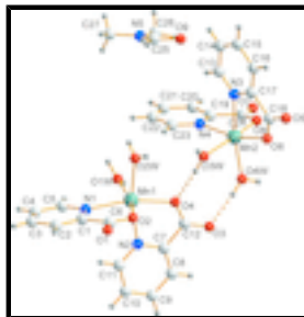
Fig. 1. The molecular structure of the title compound showing the atom-numbering scheme employed.
