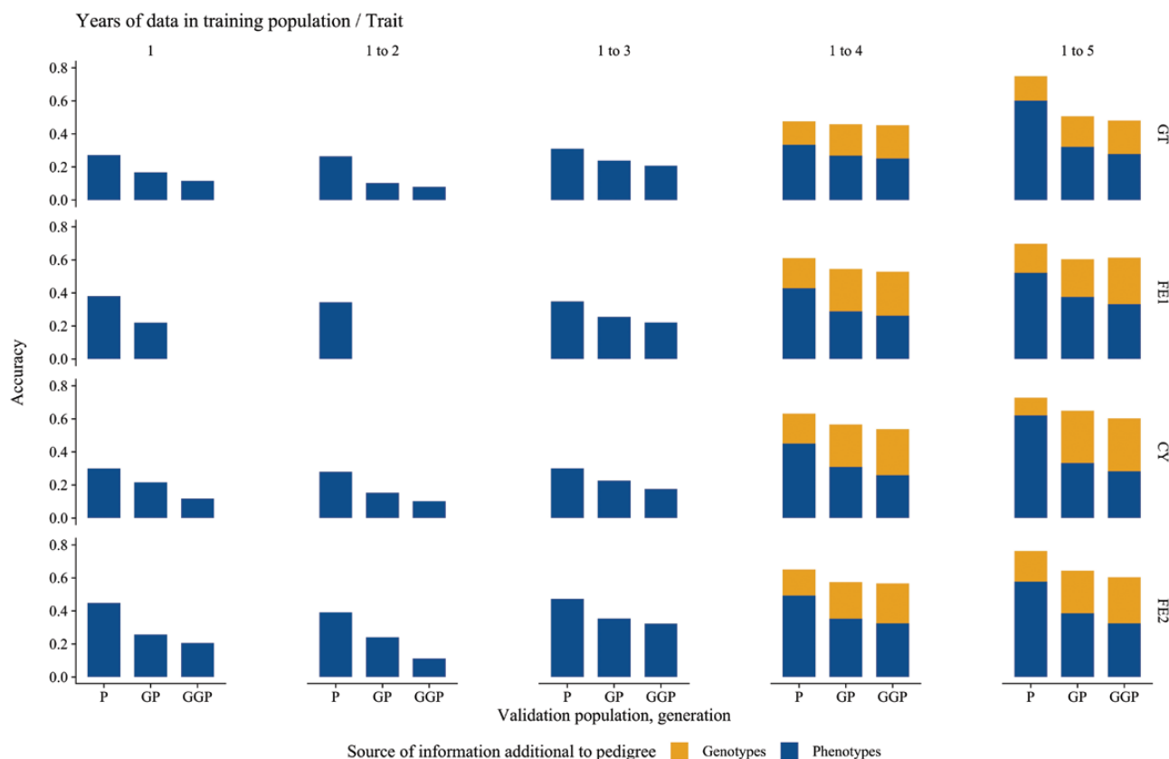
Figure 1. Trends for prediction accuracies of estimated breeding values in P, GP, and GGP of broilers in different training populations of accumulated pedigree, phenotypic, and genomic data for GT, FE1, CY, and FE2. Prediction accuracies were nearly stable with the accumulation of pedigree and phenotypes over time. The addition of genomic information generated an increase in prediction accuracy.
