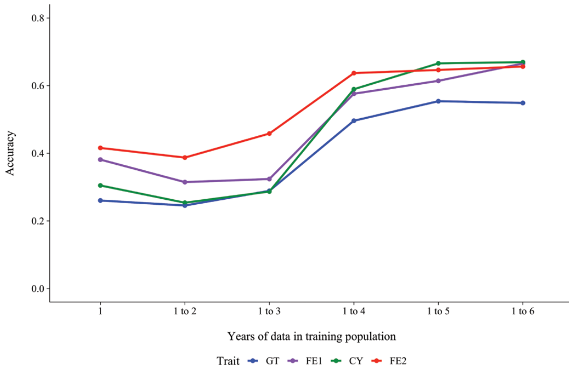
Figure 3. Trends for prediction accuracies of estimated breeding values of broilers hatched the year after the last year included in different training populations of accumulated pedigree, phenotypic and genomic data for GT, FE1, CY, and FE2. Overall, the accumulation of data increased prediction accuracy, although after accumulating data for 5 years, adding one more year of data did not increase accuracy in GT, CY, and FE2.
