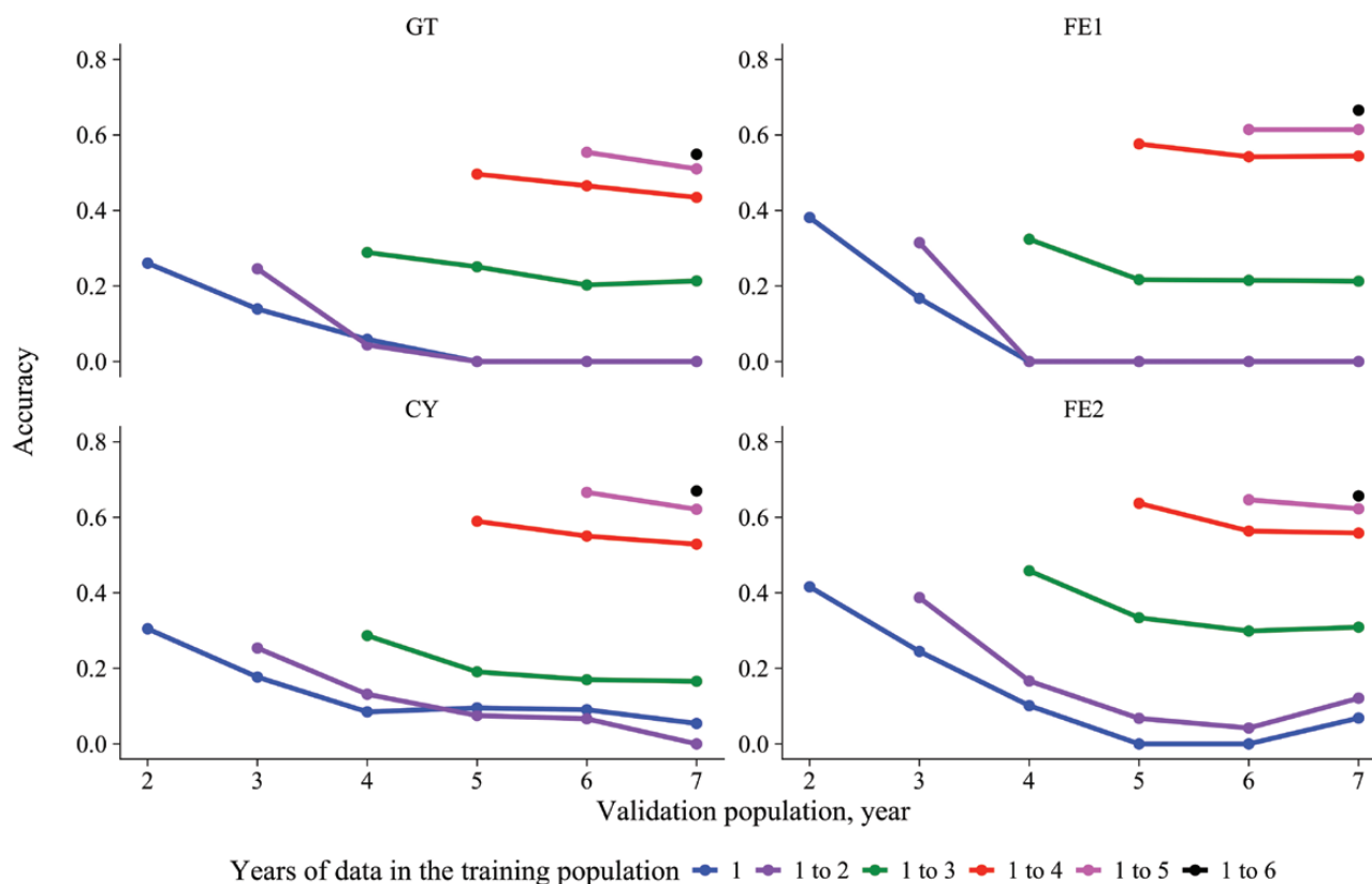
Figure 2. Trends for prediction accuracies of estimated breeding values of broilers hatched during successive years after the last year included in different training populations of accumulated pedigree, phenotypic, and genomic data for GT, FE1, CY, and FE2. Prediction accuracies were nearly stable with the accumulation of pedigree and phenotypes over time. The addition of genomic information generated an increase in prediction accuracy.
