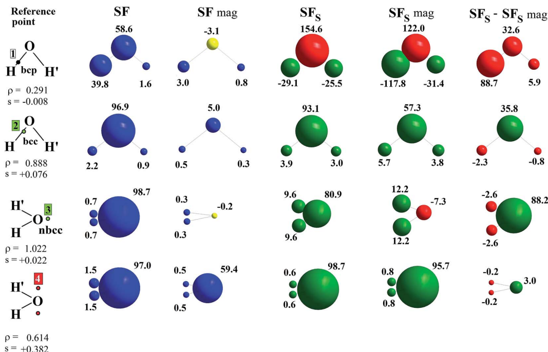
Fig. 3 SF and SF S percentage contributions at some reference points (rps) for {}^3B_1 H 2 O at the CASSCF(8,8) level. The separate contributions to SF S due to the magnetic (SF S mag) and the remaining (SF S - SF S mag) natural orbitals are also shown (for SF only those due to magnetic orbitals, denoted as SF mag). Each atom is displayed as a sphere, whose volume is proportional to the source percentage contribution to \rho(\mathbf{r}) or s(\mathbf{r}) values at the rp (first column). Colour codes: blue (yellow) atoms act as positive (negative) sources for \rho at rps; green (red) atoms act as positive (negative) sources for s at rp, hence yielding an \alpha(\beta) effect at rp (the sign of percentage source is instead positive or negative whether the atomic source concurs with or opposes s at rp).
