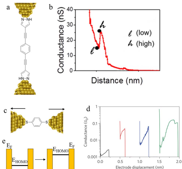
Fig. 37 (a) Schematic of 1,4-bis(1 H -pyrazol-4-ylethynyl)benzene junction; (b) a representative G - s trace obtained for 1,4-bis(1 H -pyrazol-4-ylethynyl)benzene with high and low conduction point; (c) schematic of a BDT molecular junction; (d) a representative G - \Delta z trace of BDT with spike in conductance; (e) schematic energy diagram demonstrating how the energy of the HOMO changes relative to E_F of the electrodes as electrode separation increases. Figures adapted with permission from ref. 117 and 118. Copyright 2018, American Chemical Society. Copyright 2011, Springer Nature Limited.
