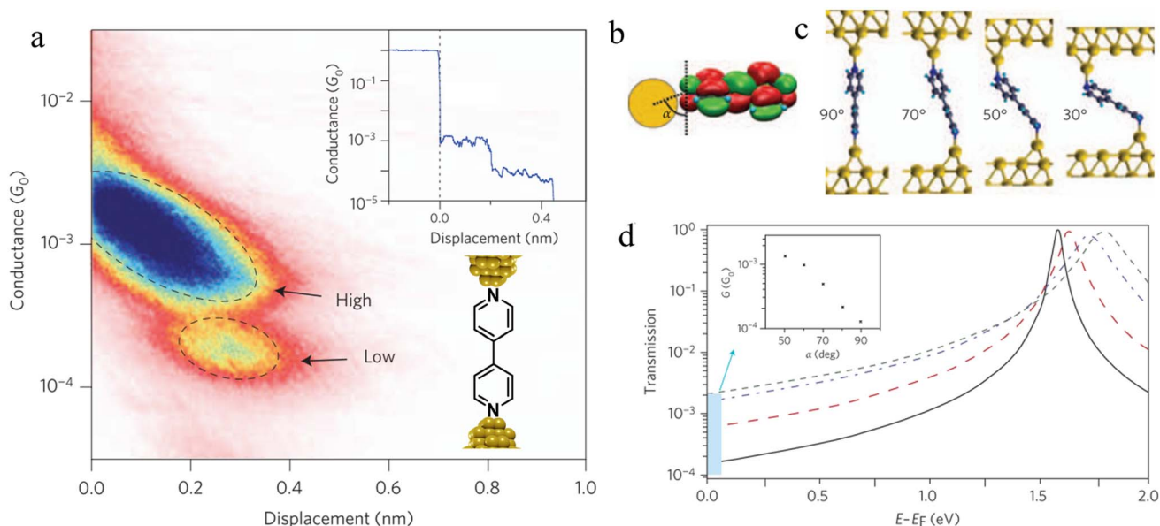
Fig. 33 (a) 2D histogram with two conductance states – high and low. Inset: example of conductance trace with two steps; (b) schematic of the coupling between the gold– s -orbital (orange) with the bipyridine LUMO where \alpha is the angle between the nitrogen–gold bond and the \pi^* -system; (c) junction geometries of bipyridine bonded on each side to gold adatoms, with varying \alpha ; (d) self-energy corrected transmission functions plotted on a semi-logarithmic scale for the junctions: black solid line for \alpha = 90^\circ , red dashed line for \alpha = 70^\circ , blue dashed–dotted line for \alpha = 50^\circ , and green dotted line for \alpha = 30^\circ . The inset shows G decreasing with increasing \alpha . Figures adapted with permission from ref. 111. Copyright 2009, Springer Nature.
